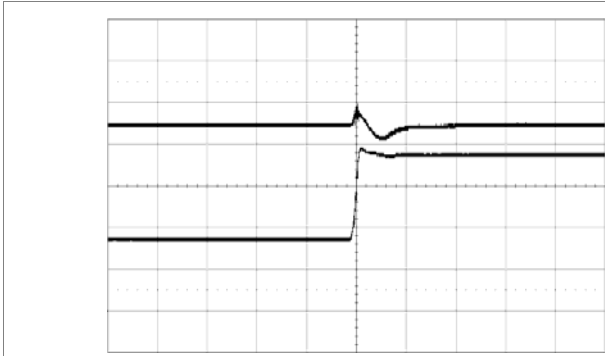
Output voltage response to input voltage transient at: T_{P1}, T_{P3} = +25^\circ\text{C}, V_I = 36\text{-}75\text{ V}, I_O = 35\text{ A} resistive load, C_O = 3.5\text{ mF} Top trace: output voltage (2 V/div.). Bottom trace: input voltage (20 V/div.). Time scale: (0.5 ms/div.).
