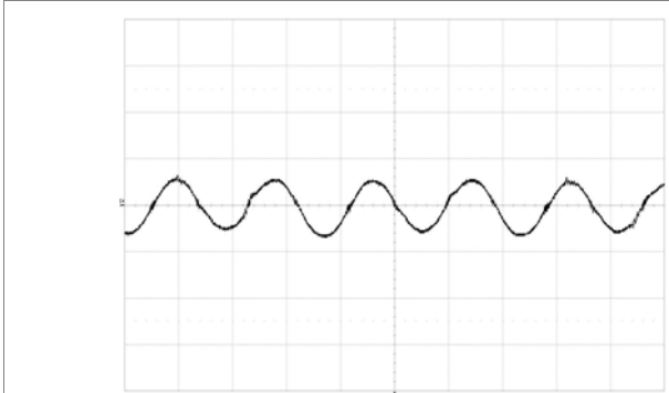
Output voltage ripple at: T_{P1}, T_{P3} = +25^\circ\text{C}, V_I = 53\text{ V}, I_O = 35\text{ A} resistive load. Trace: output voltage (50 mV/div.). Time scale: (2 μs/div.).
