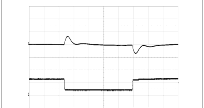
Output voltage response to load current step-change (8.75-26.25-8.75 A) at: T_{P1}, T_{P3} = +25^\circ\text{C}, V_I = 53\text{ V}, C_O = 3.5\text{ mF}. Top trace: output voltage (0.2 V/div.). Bottom trace: output current (20 A/div.). Time scale: (0.5 ms/div.).
