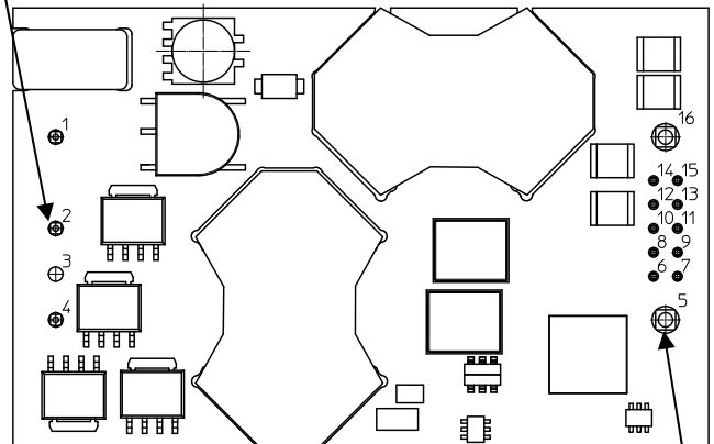
Pin 5 for measurement of minimum pin (solder joint) temperature, T_{PIN}
