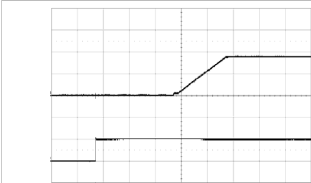
Start-up enabled by connecting V_I at: T_{P1}, T_{P3} = +25^\circ\text{C}, V_I = 53\text{ V}, I_O = 35\text{ A} resistive load. Top trace: output voltage (5 V/div.). Bottom trace: input voltage (50 V/div.). Time scale: (5 ms/div.).
